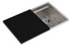
CS30BPK Stainless Steel Single Bowl Undermount Sink Kit with Black Polymer Boards Dimensions: 32-1/2" x 20-1/2" x 10" Min. Cabinet Size: 36"
